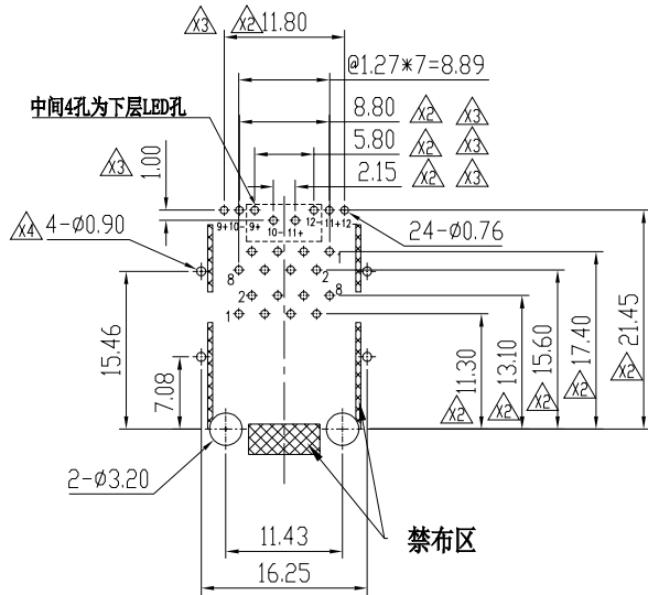
RECOMMENDED PCB LAYOUT (VIEWED FROM COMPONENT SIDE) TOLERANCE ±0.05 THICKNESS MIN=1.6MM
